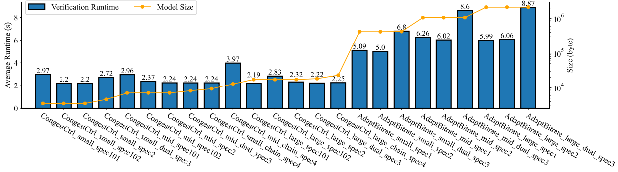
Figure 5. Verification time versus model size for CongestCtrl and AdaptBitrate. The bars represent the benchmark verification time from \alpha\beta -CROWN (the left y-axis), and the line indicates the ONNX model size in bytes (the right y-axis). The benchmarks are sorted by their model size.
