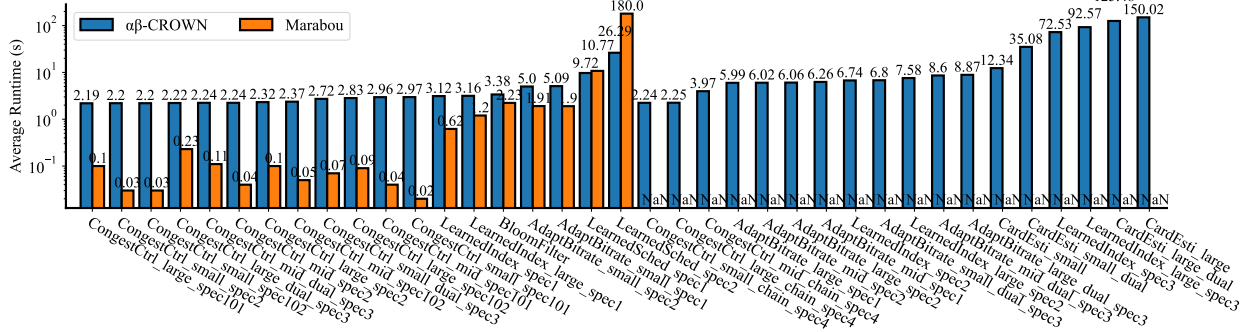
Figure 4. Verification runtime for different benchmarks. The x-axis are the benchmarks; the y-axis is the average verification runtime of ten cases (in log-scale). Bars on the left are the benchmarks solved by both verifiers; on the right are the ones only solved by \alpha\beta -CROWN. The bars are sorted by the verification time, and the exact runtime is marked on top of the bars.
