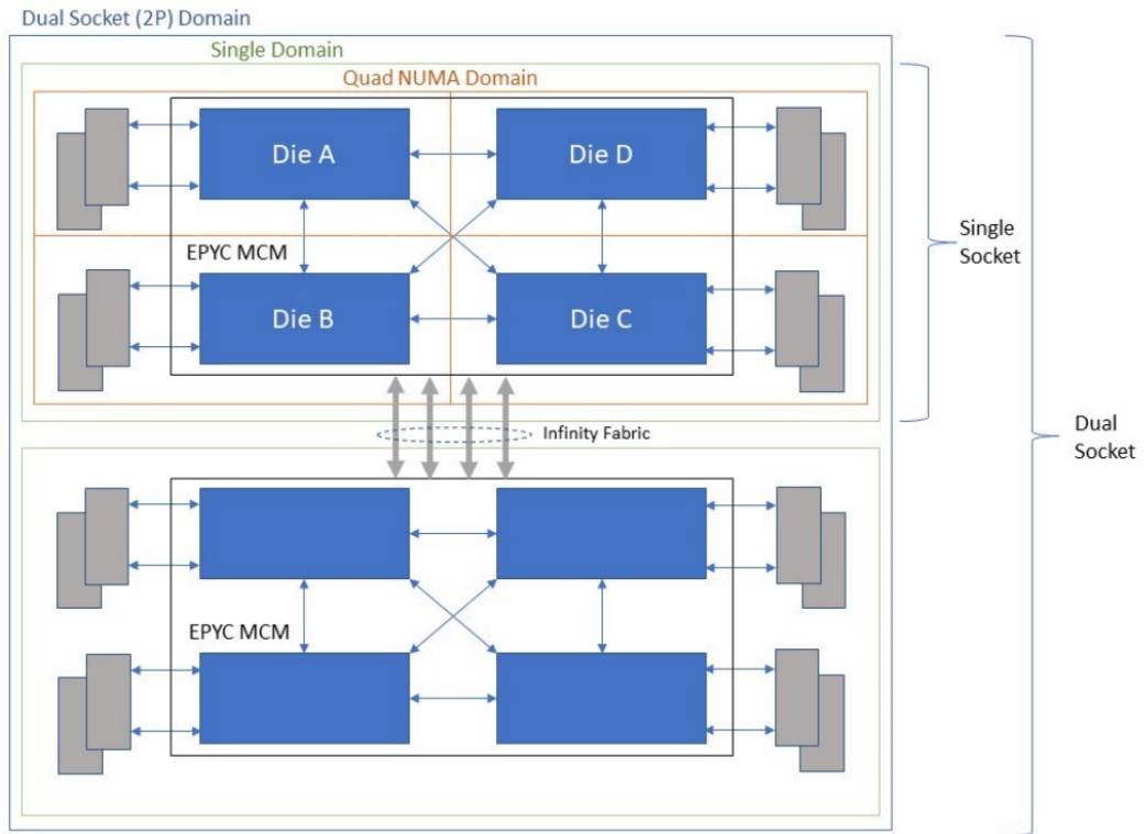
Figure 3: EPYC NUMA Domains
