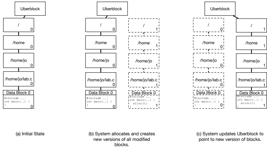
Figure 1: Copy-on-write filesystem: modifying a data block
